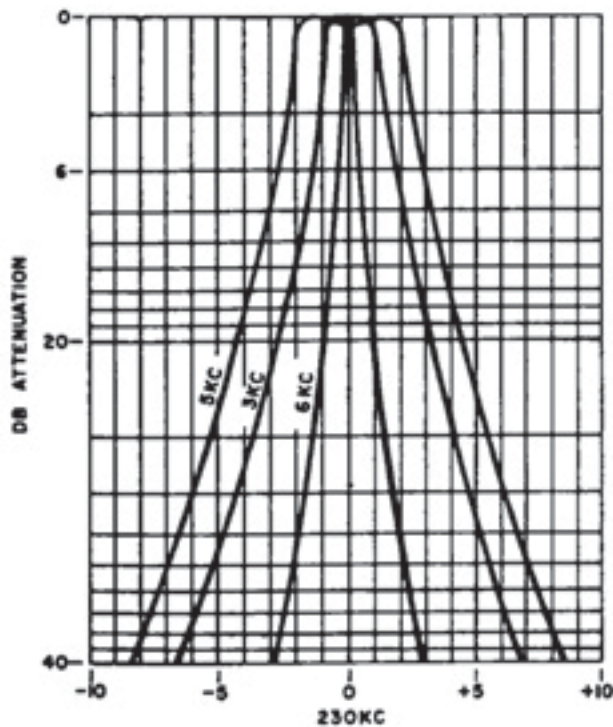
SELECTIVITY CURVES
