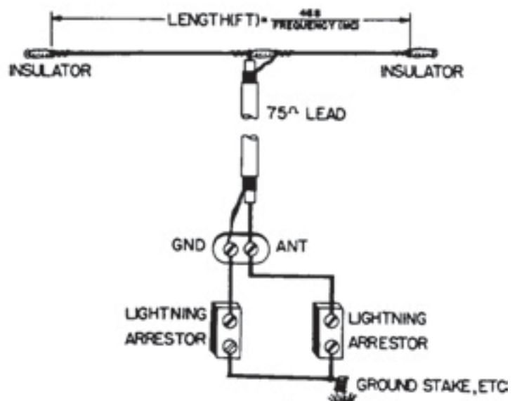
DOUBLET ANTENNA
